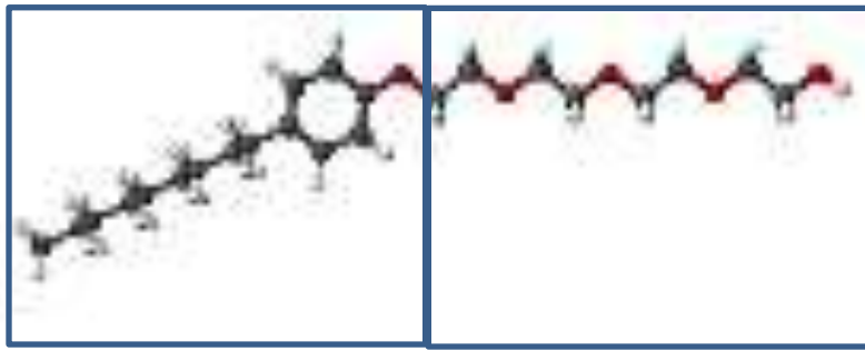
Nonylphenol
